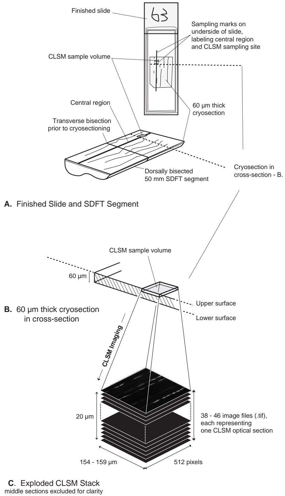
Figure 2.5 Optical Sampling
