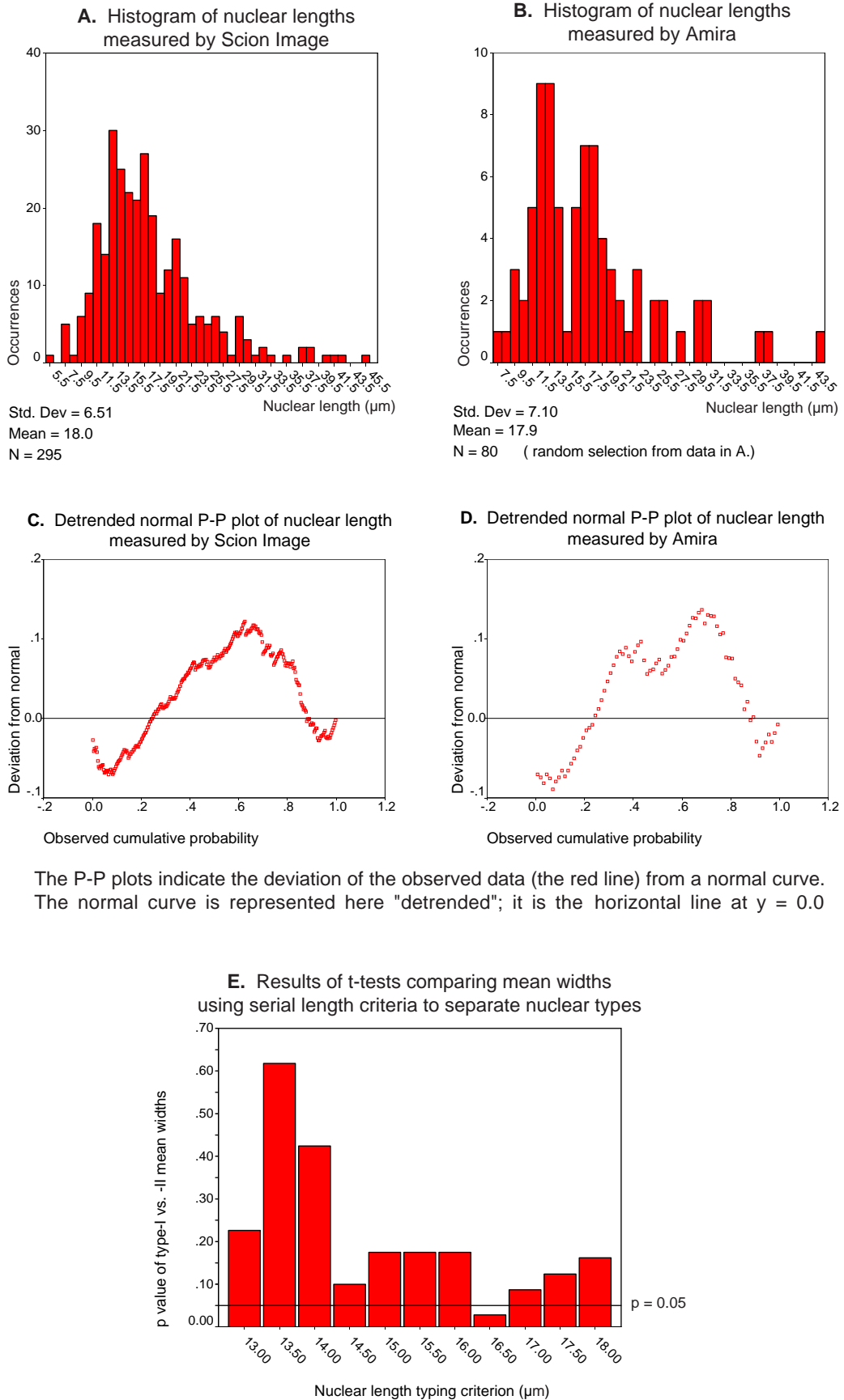
Figure 3.2 Nuclear Length Histograms and T-Test Results
